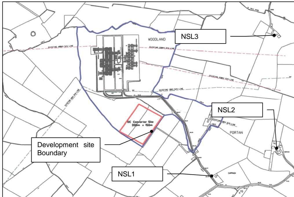
Figure 8.2 Site Layout Showing Approximate Positions of Noise Sensitive Locations
